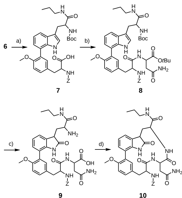
Scheme 3. Synthesis of 10 . a) 3 (1.1 equiv), [Pd(dppf)Cl 2 ]·CH 2 Cl 2 (5 mol%), K 2 CO 3 (3 equiv), DME/H 2 O (7:1), 70 °C; b) H-Asn-OrtBu, EDCI, HOBT; c) DMSO (20 equiv), AcOH/HCl (4:1); d) PyBOP (4 equiv), HOBT (4 equiv), DIEA (6 equiv). PyBOP = benzotriazol-1-yloxytripyrrolidinophosphonium hexafluorophosphate, DIEA = diisopropylethylamine.
